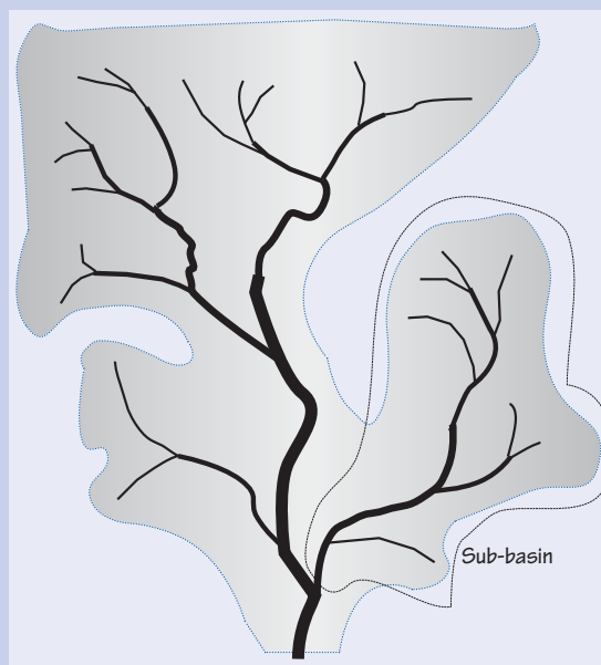
Figure 1.3 b Catchment Basins The stream system drains a catchment basin which may contain smaller sub-basins or local watersheds.
